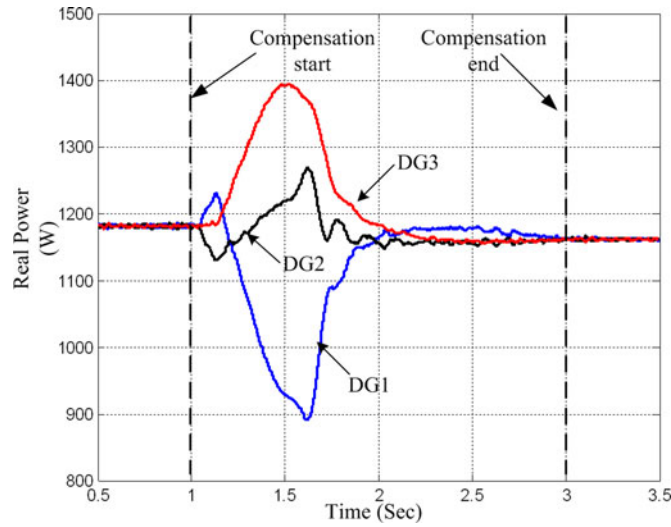
Fig. 17. Simulated real power sharing performance in a network microgrid (0.1 s synchronization flag delay in DG unit1).
