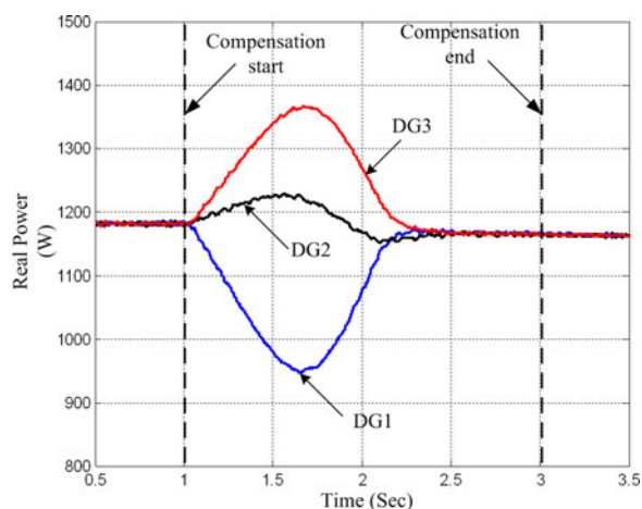
Fig. 11. Simulated real power sharing performance in a network microgrid (compensated is activated at 1 s).
